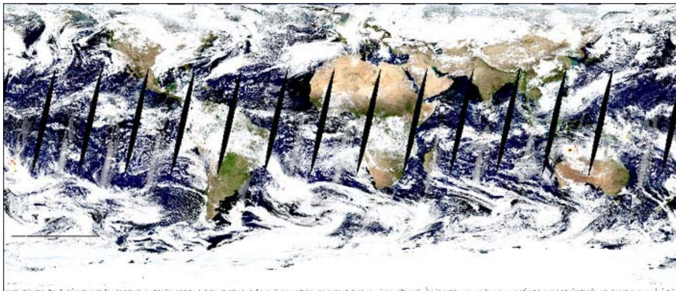
Figure 7. A MOD09CMG RGB-image composed of surface reflectance data measured by bands 1 (red), 4 (green) and 3 (blue) on December 7, 2000. The MODIS product granule ID is MOD09CMG.A2000341.005.2006347161131.hdf.
