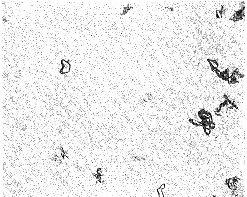
147 I4 Miscellaneous \times 18
