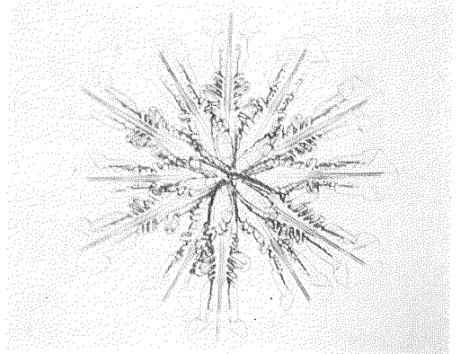
67 P3a Broad branch crystal with 12 branches \times 32
