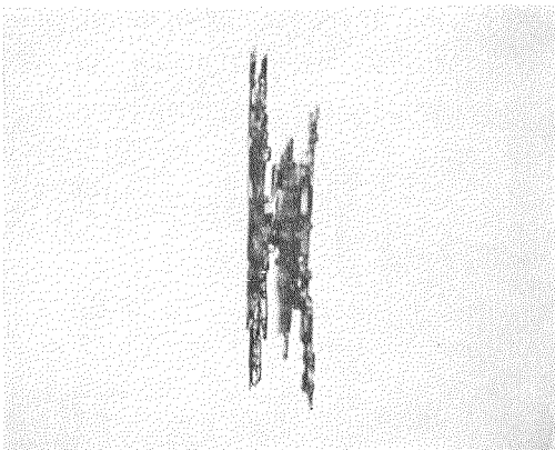
4 N1b Bundle of elementary needles × 35
