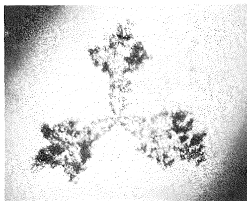
63 P2b Three-branched crystal × 30
