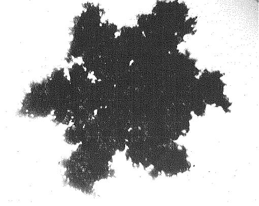
131 R3a Graupellike snow of hexagonal type \times 17
