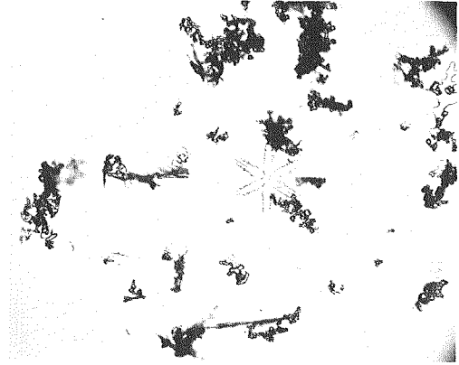
143 I2 Rimed particles \times 17
