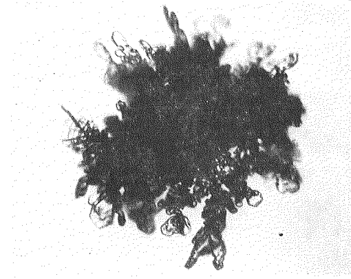
135 R3c Graupellike snow of nonrimed extensions \times 26
