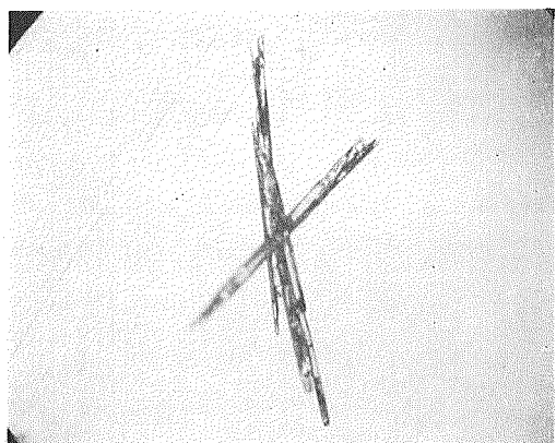
5 N2a Combination of needles × 29
