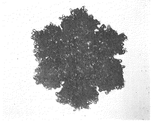
137 R4a Hexagonal graupel \times 26
