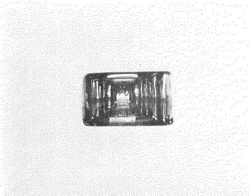
32 C1h Thick plate of skelton form \times 71
