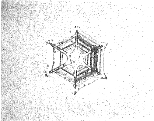
118 R1c Rimed plate \times 34
