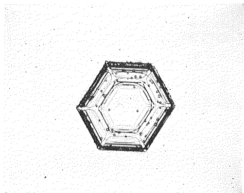
117 R1b Rimed thick plate \times 34
