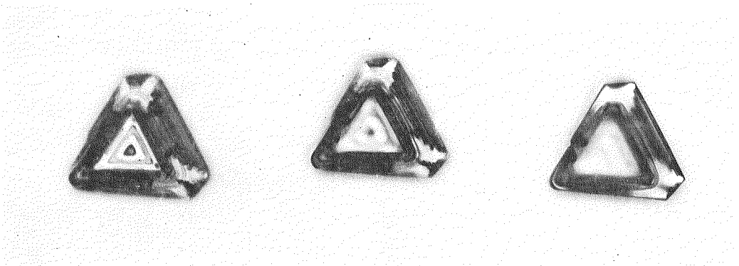
17 C1a Pyramid; focusing on top focusing on middle focusing on bottom × 73.5
