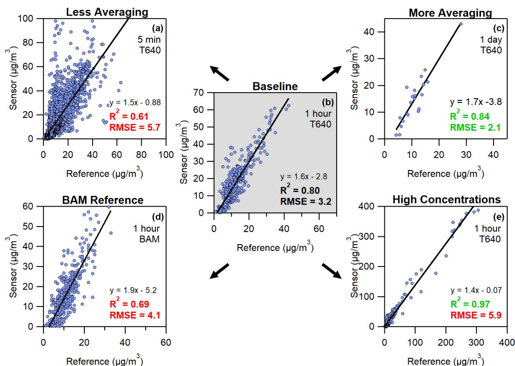
Figure 3. The changes to R^2 and RMSE from a baseline condition depending on evaluation conditions. Panel (b) shows the baseline of 1 h averaged data with T640 as a reference instrument and without 3 d of high concentrations. Panels (a) and (c) show the impact of less and more data averaging, respectively. Panel (d) shows the impact of switching to the BAM instead of the T640. Panel (e) shows the effect of high concentration by including 3 additional days during which higher concentrations were observed.
