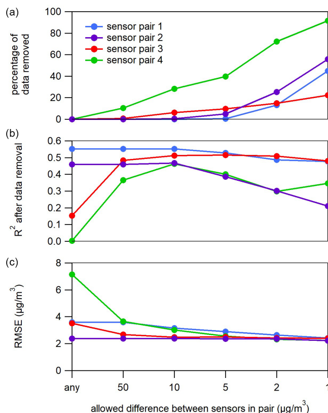
Figure 1. The eight sensor replicas were divided into four pairs with different measurement agreement requirements for the data from the sensors in each pair (first averaged to 1 h intervals). The x axis shows the allowed difference between paired measurements. Panel (a) shows the percentage of data removed from the sensor pair for different data agreement requirements. Panel (b) shows how R^2 between the sensor pair (average of the pair) and reference measurements changes when these disagreeing data points are removed. Panel (c) shows how RMSE is impacted as disagreeing data points are removed.
