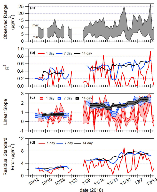
Figure 6. Linear regression parameters from 1 h measurements over a 2-month period in 2018. Panel (a) shows the range of measurements observed on each day. Panels (b)–(d) show the R^2 , slope, and residual standard error, respectively. In (b)–(d) a rolling collection of 1, 7, or 14 d of data was used to find linear regression parameters.
