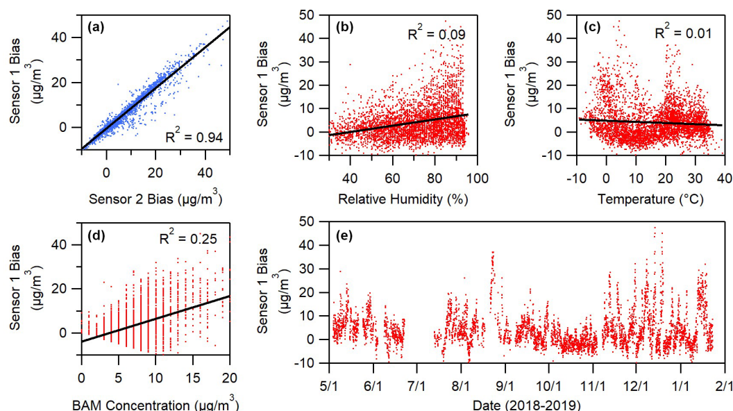
Figure 2. Panel (a) shows the correlation between the bias ( C_{\text{sensor}} - C_{\text{reference}} ) of two sensor replicas. Panels (b)–(d) show correlation between sensor bias and meteorological factors. Panel (e) shows that bias varies over time but not in a consistent pattern. Measurement gaps in (e) are the result of the BAM not meeting its internal relative humidity specification (35 %).
