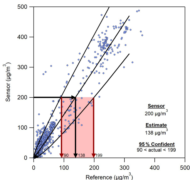
Figure 4. An example of a prediction interval evaluation for 5 min data from a single sensor in April 2019 that includes periods of high concentration. The curved lines are the upper and lower limits of the 95 % prediction interval. A visual interpretation of a new sensor measurement of 200 \mu\text{g m}^{-3} is also shown.
