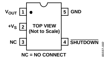
Figure 2. R-5 (SOT-23)
