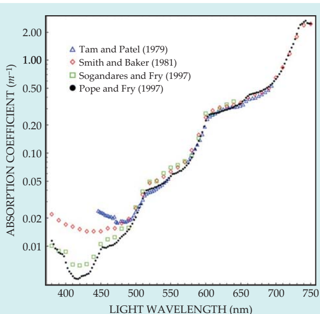
Figure 1. Various measurements of the absorption coefficient of light in pure water. Considerable discrepancy is evident near the absorption minimum at 420 nm in the blue region of the visual spectrum, where light can travel more than 100 meters with little absorption, making laboratory measurement difficult. The most accurate measurements near the minimum to date are by Edward Fry's group at Texas A&M University. 18
