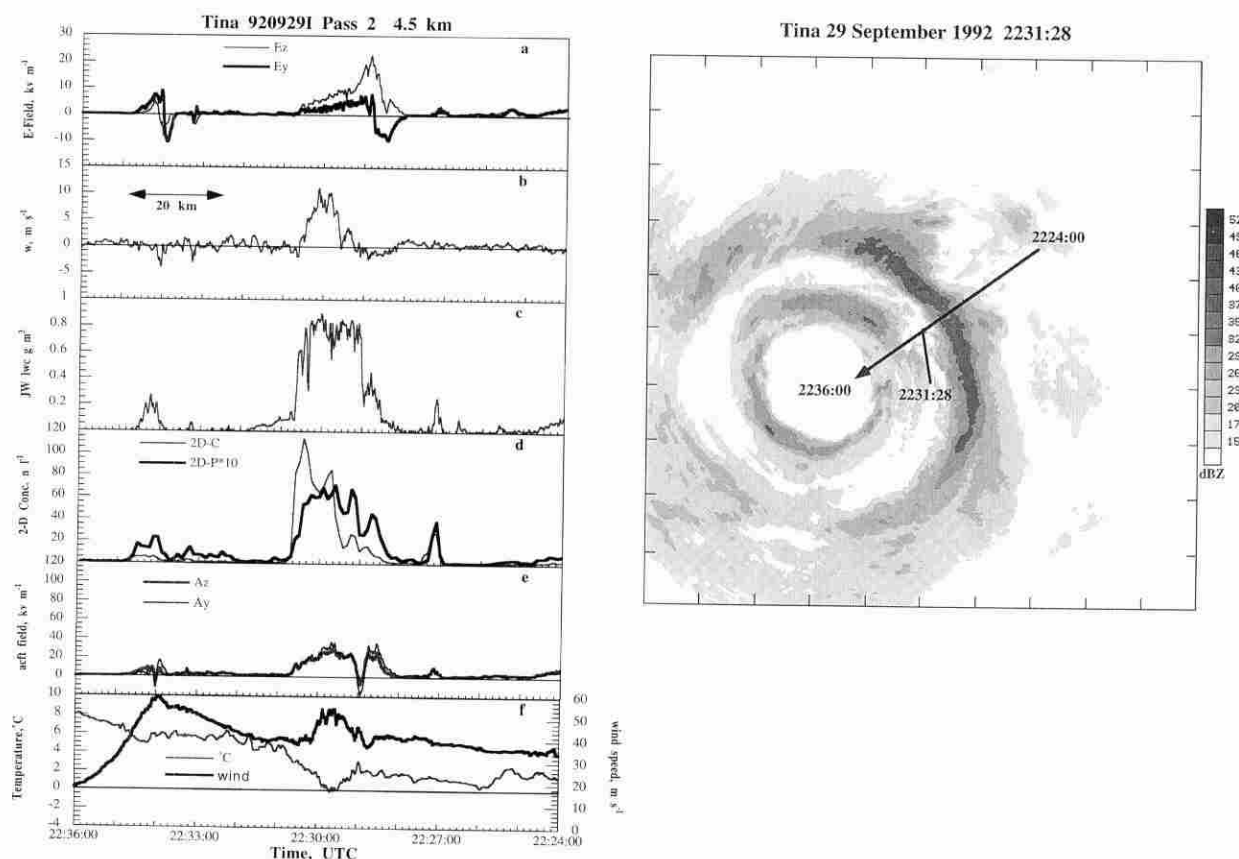
FIG. 5. Flight-level data from Hurricane Tina, 29 September 1992, from the inbound 4.5-km altitude ( +2^{\circ}\text{C} ) pass from 2224:00 to 2236:00. (a) Vertical ( E_z ) and horizontal ( E_y ) E components ( \text{kV m}^{-1} ); (b) vertical velocity ( \text{m s}^{-1} ); (c) cloud liquid water content from the JW probe ( \text{g m}^{-3} ); (d) particle number concentration ( \text{L}^{-1} ) deduced from 2D particle image data. The precipitation probe number concentration is multiplied by 10 for clarity. (e) Vertical and horizontal aircraft field ( \text{kV m}^{-1} ) from both pairs of field mills; (f) temperature and horizontal wind speed. (Radar) Single-sweep PPI reflectivity display from the WP-3D lower fuselage radar. The start and end points of the pass are as shown by the long arrow. The aircraft position at the time of the radar image is marked.
