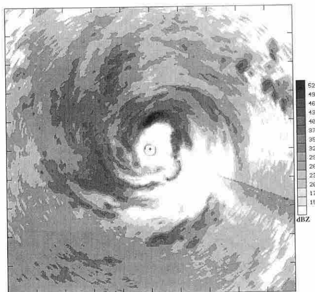
FIG. 4. Single-sweep PPI map of Hurricane Claudette at 1628:27. North is toward the top of the figure. The aircraft penetrated the storm along a northwest-southeast track. The strong convective cell in which the strongest E and most lightning flashes were encountered is in the north eyewall. In this and all subsequent radar images, the aircraft position at the time the image was obtained is marked with a + . The blanked-out area around the + is caused by the range delay of the radar, and the ring of return around the + is where the side-lobe return from the sea surface appears.
