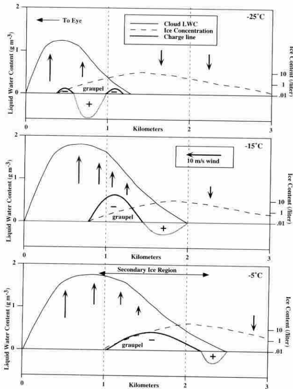
FIG. 15. Idealized cross section through the upshear side of an updraft containing supercooled liquid water and a downdraft containing ice-containing downdraft as might occur in a hurricane eyewall (with circular symmetry) or locally in a deep convective cloud. The charge separation protocol was taken from Saunders et al. (1991; Fig. 7); other scenarios are possible. Arrows indicate local vertical velocity, and the expected location of graupel particles is shown. Separation of charge resulting from ice-graupel collisions depends on the relative concentration of particles and the magnitude of the liquid water content; the sign and magnitude of the charge on the target (larger) particle is indicated, as inferred from laboratory data. The sign and magnitude of the separated charge varies with location both along the horizontal (as measured by aircraft penetrations perpendicular to the horizontal wind) and in the vertical (from aircraft penetrations at different temperatures). The relative concentration of vapor-grown ice results from splinter production by the Hallett-Mossop process under appropriate conditions. Subsequent vertical and downdraft advection of the particles determines the LWC to ice transition. The charging processes are controlled by the rate at which splinters are captured by supercooled drops to form new rimers and produce yet more splinters under appropriate conditions and the rate of bounce of such particles from growing graupel.
