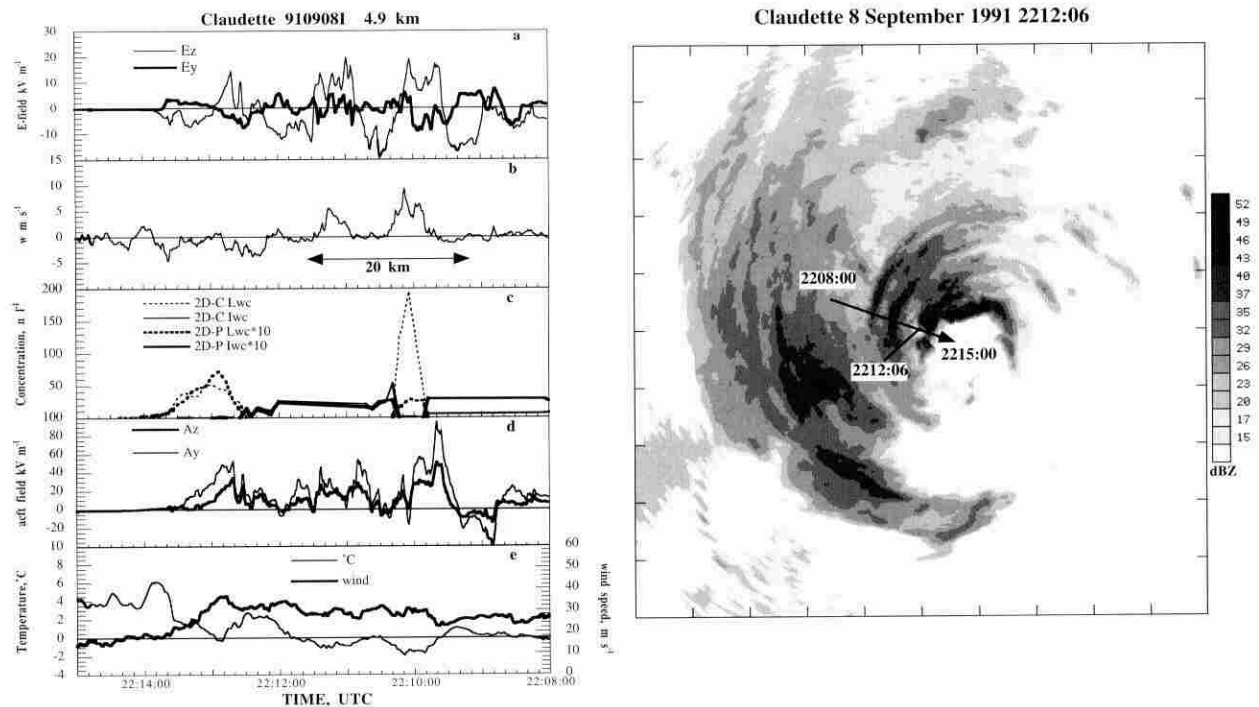
FIG. 8. As in Fig. 7 but for the 4.9-km ( +2^{\circ}\text{C} ) inbound pass from 2208:00 to 2215:00. Sunset occurred at 22:10:00, and lightning flashes were observed at \sim 2209 and \sim 2210 . (a) Vertical and horizontal electric field ( \text{kV m}^{-1} ); (b) vertical velocity ( \text{m s}^{-1} ); (c) two-dimensional particle image number concentration ( \text{L}^{-1} ) by particle phase. The 2D-P values are multiplied by 10 for clarity. (d) Vertical and horizontal aircraft field ( \text{kV m}^{-1} ); temperature ( ^{\circ}\text{C} ) and horizontal wind speed ( \text{m s}^{-1} ). (Radar) Single-sweep PPI reflectivity display from the WP-3D lower fuselage radar. The start and end points of the pass are as shown by the long arrow. The aircraft position at the time of the radar image is marked.
