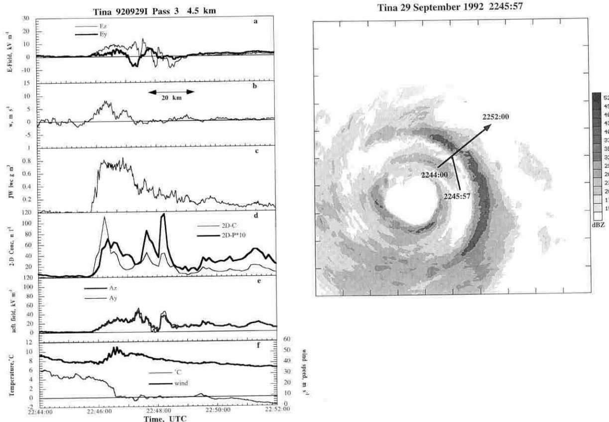
FIG. 6. As in Fig. 5 but for the reciprocal outbound pass from 2244:00 to 2252:00 (0°C). (a) Vertical ( E_z ) and horizontal ( E_y ) E components ( \text{kV m}^{-1} ); (b) vertical velocity ( \text{m s}^{-1} ); (c) cloud liquid water content from the JW probe ( \text{g m}^{-3} ); (d) particle number concentration ( \text{L}^{-1} ) deduced from 2D particle image data. The precipitation probe number concentration is multiplied by 10 for clarity. (e) Vertical and horizontal aircraft field ( \text{kV m}^{-1} ) from both pairs of field mills; (f) temperature and horizontal wind speed. (Radar) Single-sweep PPI reflectivity display from the WP-3D lower fuselage radar. The start and end points of the pass are as shown by the long arrow. The aircraft position at the time of the radar image is marked.
