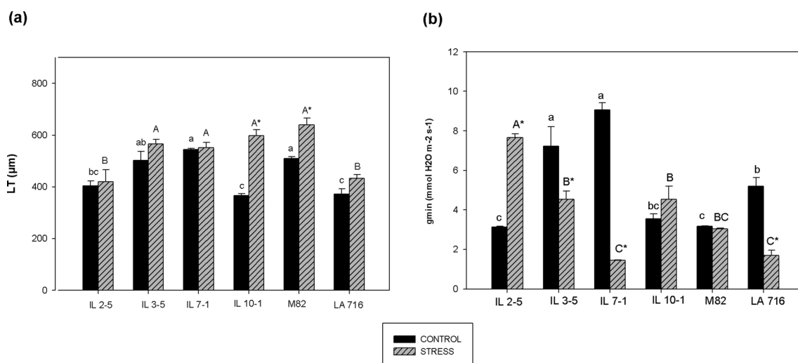
Figure 3. Leaf thickness (LT) (a) and minimum epidermal conductance ( g_{\text{min}} ) (b) of tomato genotypes grown under two different water regimes (50 and 100% ASW), quantified on top third leaves, 60 days after the beginning of the stress treatment. Same lower- and upper-case letters indicate that the genotypes did not differ by the Tukey's test ( p > 0.05 ), in the control (100% ASW), and in the stress treatment (50% ASW), respectively. The asterisk (*) indicates statistical difference between control and stress treatment for the same genotype. Data are expressed as means ± standard error.
