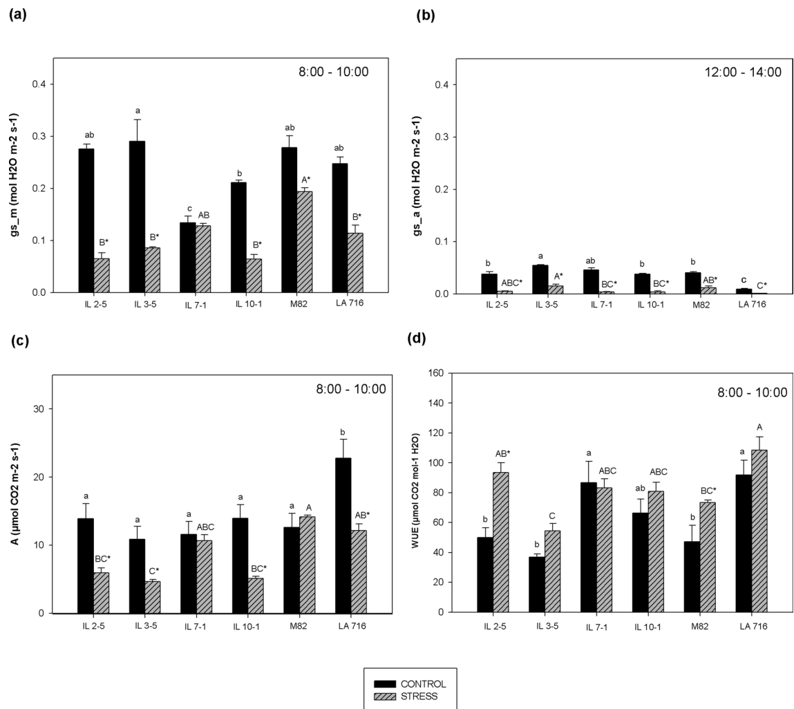
Figure 2. Physiological traits stomatal conductance in the morning (8:00–10:00) ( g_{s\_m} ) (a) and in the afternoon period (12:00–14:00) ( g_{s\_a} ) (b), photosynthesis (A) (c), and water use efficiency (WUE) (d) of tomato genotypes grown under two different water regimes (50 and 100% ASW), quantified on top third leaves, 60 days after the beginning of the stress treatment. A was recorded only in the morning period. WUE was expressed as A/g_s ratio in the morning period. Same lower- and upper-case letters indicate that the genotypes did not differ by the Tukey's test ( p > 0.05 ), in the control (100% ASW), and in the stress treatment (50% ASW), respectively. The asterisk (*) indicates statistical difference between control and stress treatment for the same genotype. Data are expressed as means \pm standard error.
