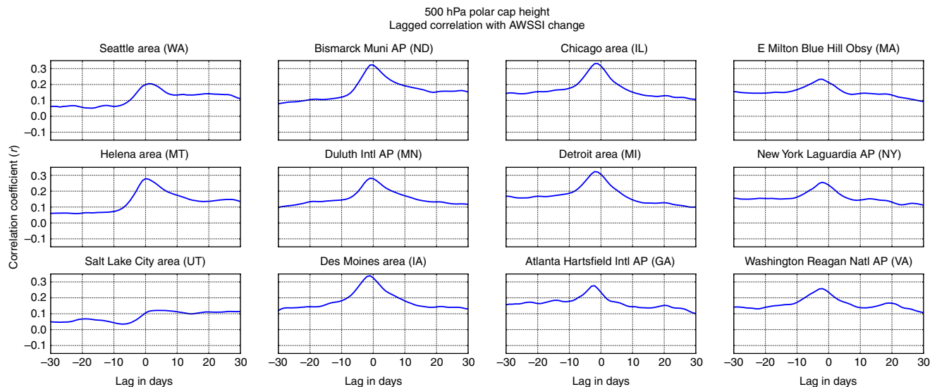
Fig. 5 Arctic variability leads occurrence of severe winter weather. The correlation between average daily change in the AWSSI at selected weather stations across the US associated with polar cap geopotential height anomalies (PCH) for all days between \pm 30 days. The peak value is reached when the PCH leads the AWSSI by 5 days
