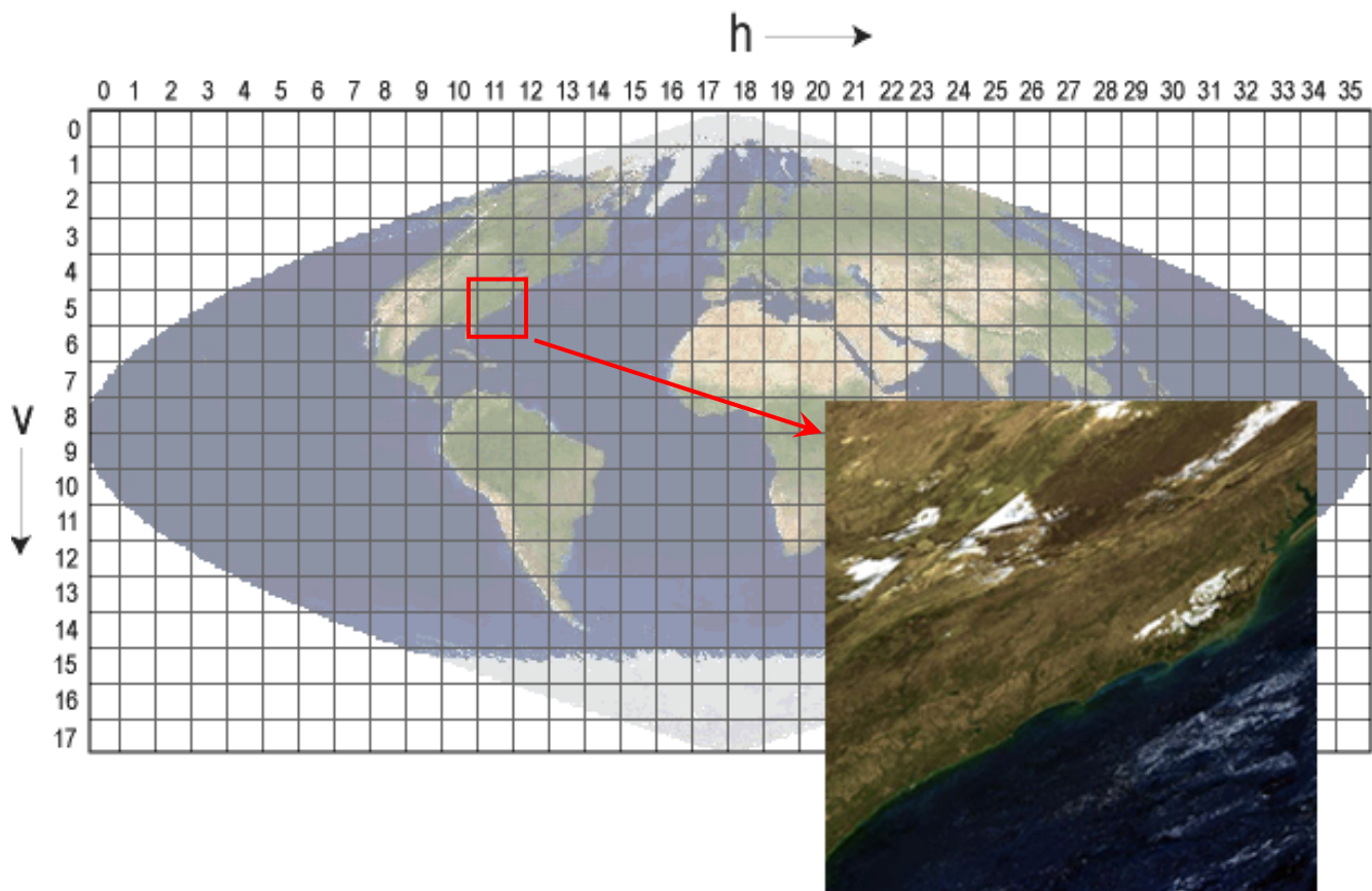
Figure 1. The MODIS sinusoidal grid consists of 460 nonoverlapping tiles which measure approximately 10^\circ \times 10^\circ . Data from an example tile (tile h11v05, derived from MOD09A1.A2000337.h11v05.005.2006342055602.hdf) is shown as a RGB-image.
